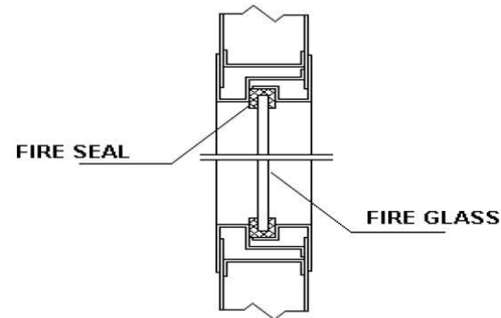
DETAIL OF VISION PANEL
