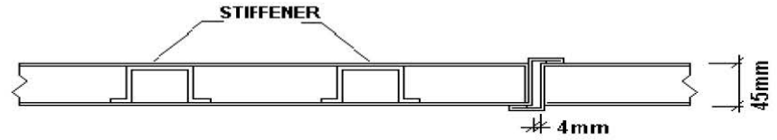
MEETING STILE : STIFFENER DETAIL
