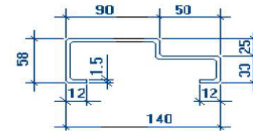
STEEL FRAME PROFILE 1.5 E.G.
